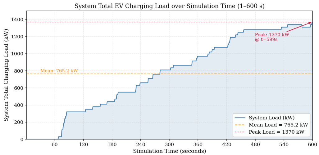
Figure 4.1: System total charging load over simulation time (1–600 seconds).
